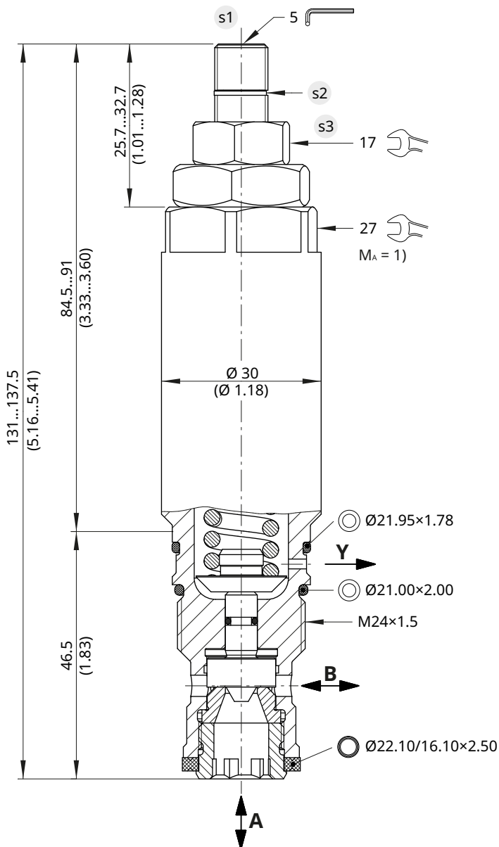
Version "S": Einstellschraube (Standard) Version "S": adjustment screw (standard)
