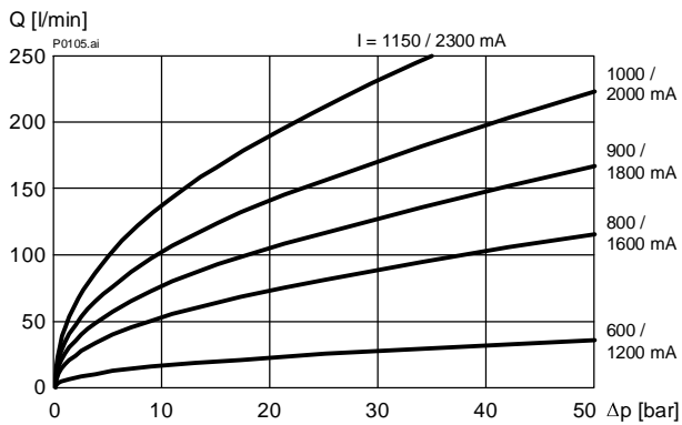
Q = f (Δp; I) Flow rate adjustment characteristic [„140“]
