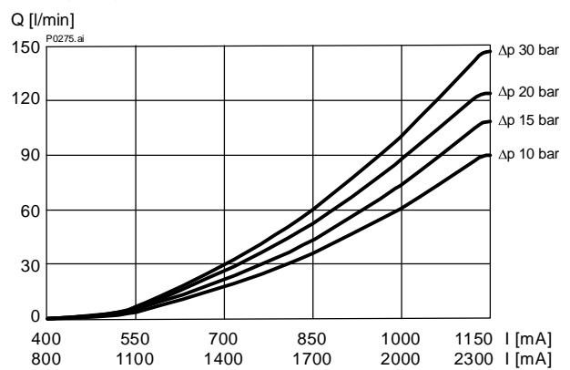
Q = f (I; Δp) Flow rate adjustment characteristic [„90“]
