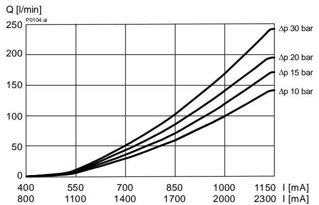
Q = f (I; Δp) Flow rate adjustment characteristic [„140“]
