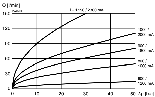
Q = f (Δp; I) Flow rate adjustment characteristic [„90“]
