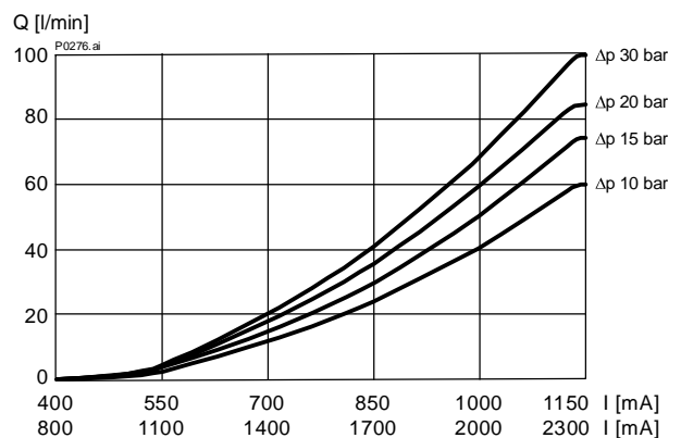
Q = f (I; Δp) Flow rate adjustment characteristic [„60“]
