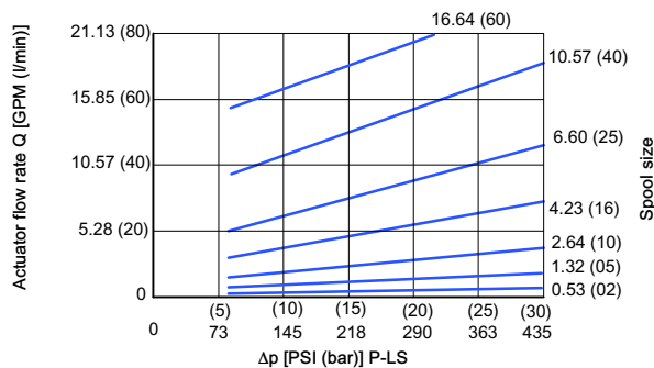
5.2.4.3 LD/LC Maximum flow rate at the directional valve without compensator function, LS-function
